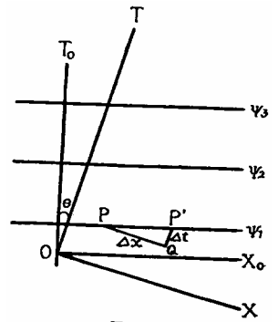
FIG. 2 (From Wave Mechanics , by H. F. Biggs)
